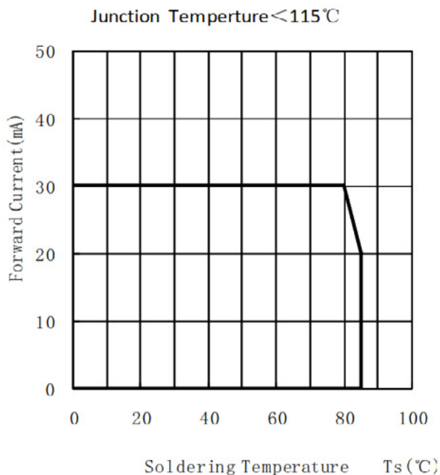
Soldering Temperature vs. Forward Current
